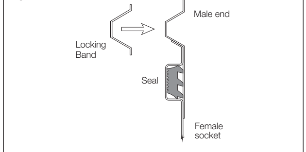
Fig. 5 Standard Joint detail
